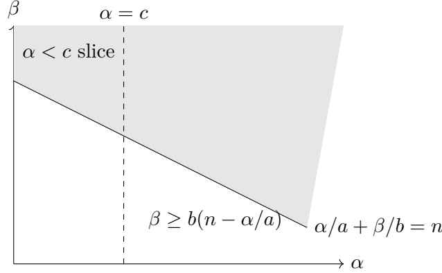
FIGURE 9. Generators of (x^c, \overline{I^n}) correspond to lattice points above the line, truncated by \alpha < c ; the count is eventually linear in n .
