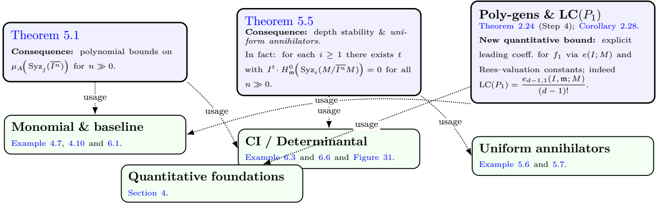
FIGURE 4. Result-Example Map (headlines → theorems → usage): compact visualization.
