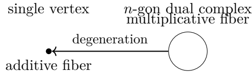
Figure 27: Geometric jump across the reduction-type boundary: the dual complex collapses from an n -gon to a single component, causing a discontinuous change in the conductor and local L -factor.
