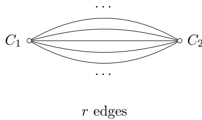
Figure 28: Dual graph for Example 6.1 : two vertices joined by r edges; \beta_1(\Gamma) = r - 1 .
