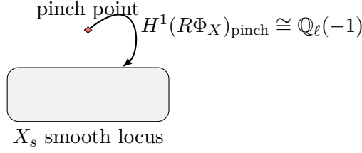
Figure 31: Failure of strict semistability: vanishing cycles at a pinch point inject a wild \mathbb{Q}_\ell(-1) into H^2(X) , violating H^2(X)^{I_K} \cong H^2(X_s) .
