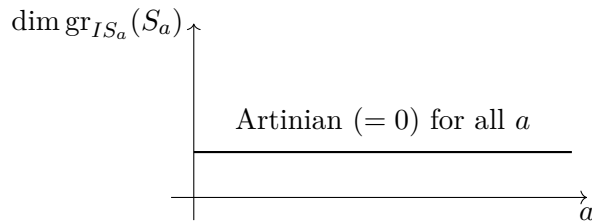
FIGURE 33. Monomial deformation x^2 = t : constant (Artinian) fiber dimension = 0; nilpotents appear at a = 0 but USC holds.
