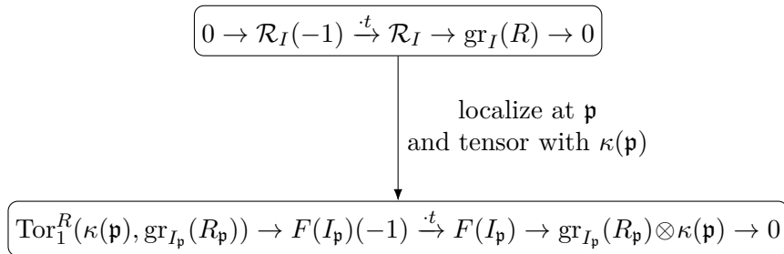
FIGURE 37. Fiber exact sequence. Nonzero \ker(\cdot t) in degree 1 \iff degree-1 zero-divisor in F(I_{\mathfrak{p}}) (dense on the base), forcing \text{Ass}(\text{gr}_I) to be dense.
