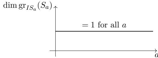
FIGURE 32. Determinantal family xz = ay^2 : constant \dim(\mathrm{gr}) = 1 ; the degree-1 torsion locus is constructible, compatible with USC.
