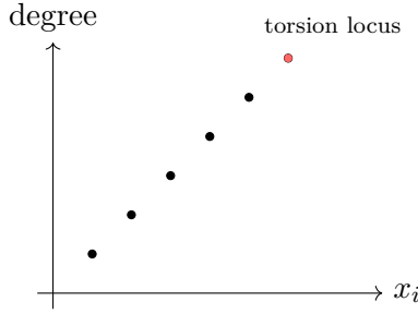
FIGURE 23. Visualization of the fiberwise degree-1 torsion locus: points (x_i, \deg) denote generators along the Rees valuation scale. The highlighted red point indicates the emergence of torsion in degree 1, triggering the Zariski-dense behavior of \text{Ass}(\text{gr}_I(R)) described in Proposition 2.14 .
