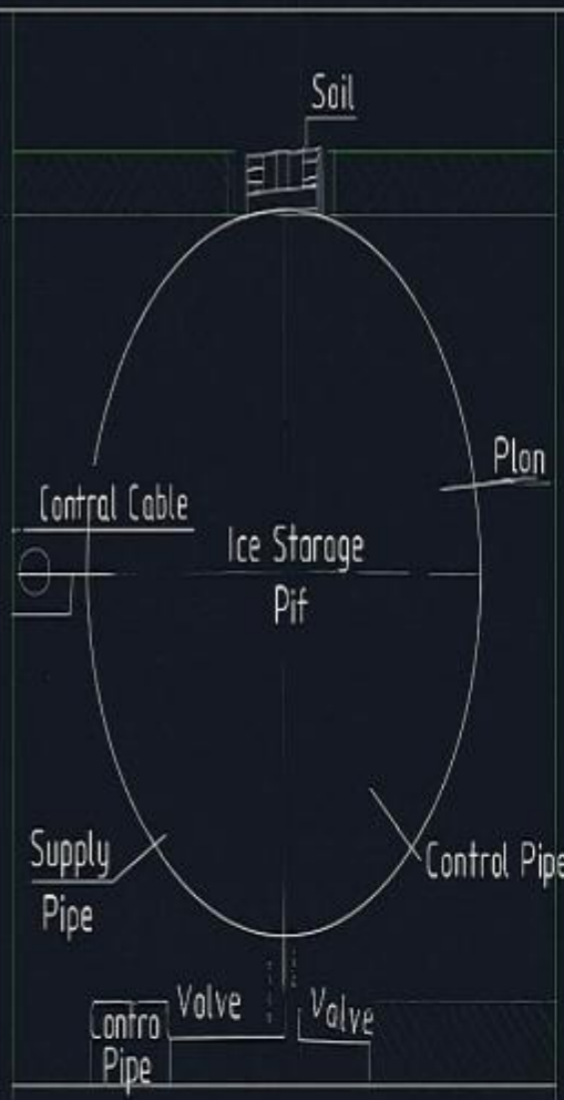
Plan View
