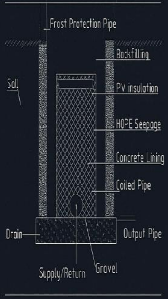
Section View
