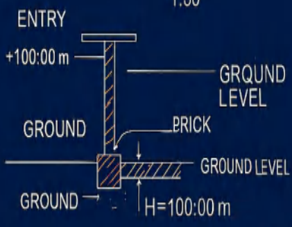
SECTION A
