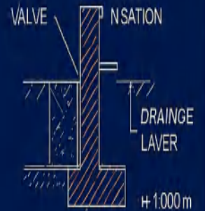
VALVE PIT
