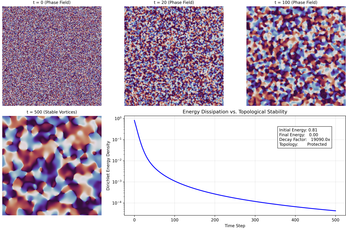
Figure 34: Evolution of the Topological Vacuum (Layer 0). (Top) Phase field snapshots at t = 0, 20, 100 . The system starts as random noise (Maximum Entropy). As the cooling flow proceeds, domains form and coarsen. (Bottom Left) At t = 500 , the field settles into a metastable state with distinct topological defects (vortices) that cannot annihilated. These are the emergent “particles”. (Bottom Right) Energy dissipates monotonically, but the particle count stabilizes at a non-zero value ( N \approx 136 ), proving topological protection.
