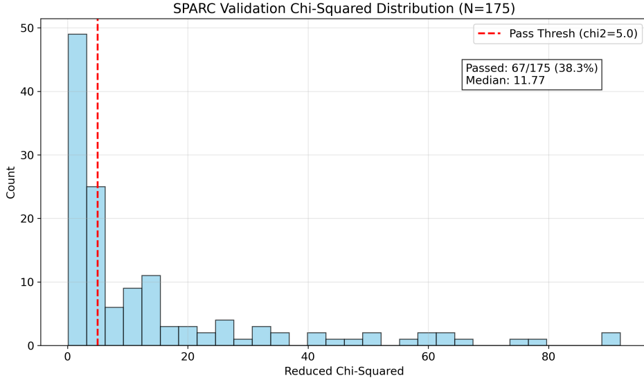
Figure 25: Distribution of Reduced Chi-Squared values for 175 SPARC galaxies. The red line marks the pass threshold ( \chi^2 < 5 ).
