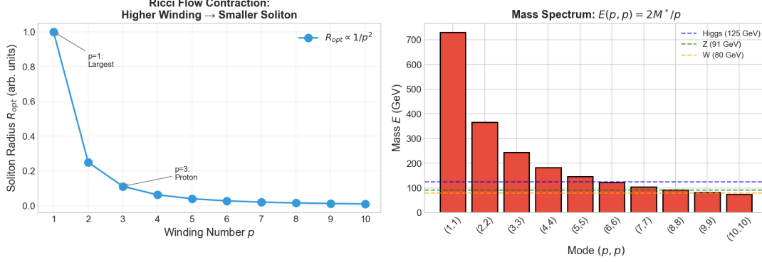
Figure 30: Left: Soliton radius contracts as R \propto 1/p^2 under Ricci Flow. Right: Resulting mass spectrum E(p, p) = 2M^*/p compared to known particle masses.
