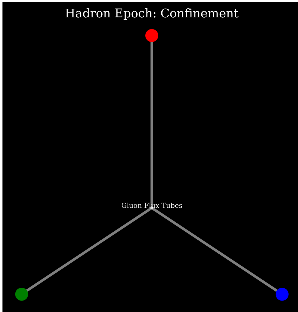
Figure 4: Hadronization process.
