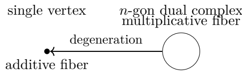
Figure 24: Geometric jump across the reduction-type boundary: the dual complex collapses from an n -gon to a single component, causing a discontinuous change in the conductor and local L -factor.
