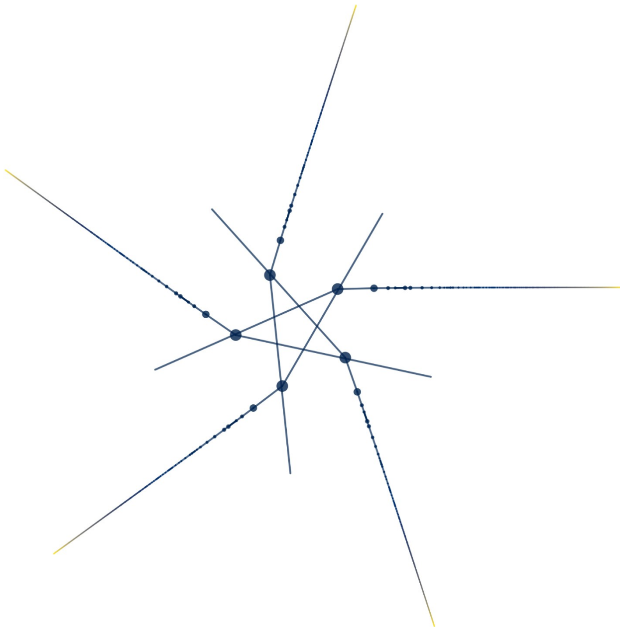
Figure 6: Generative Art from Complex Keçeci Numbers
