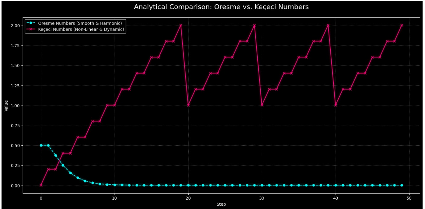
Figure 8: Analytical Comparison Oresme vs. Keçeci Numbers
