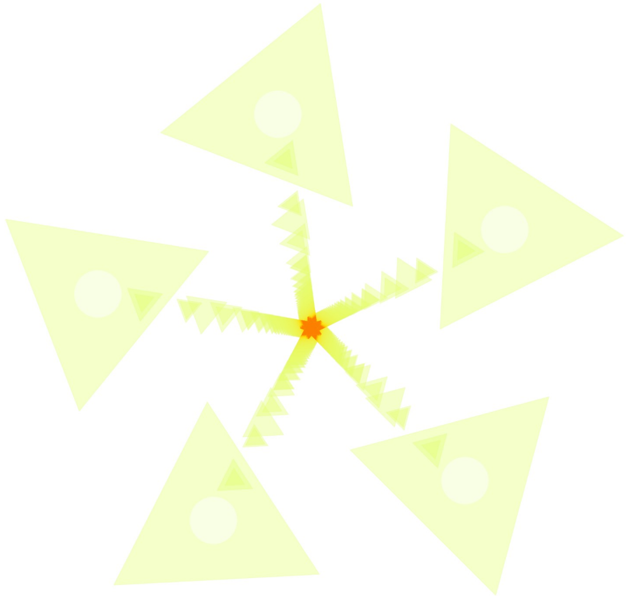
Figure 7: Generative Art from Complex Keçeci Numbers
