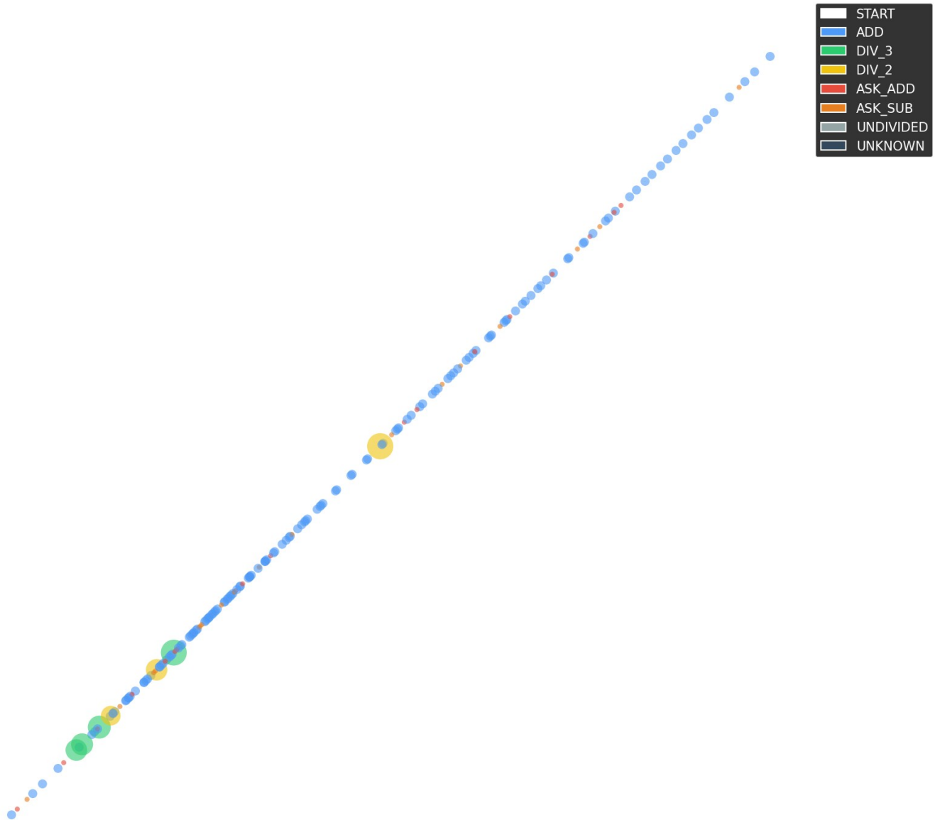
Figure 4: Generative Art from Complex Keçeci Numbers
