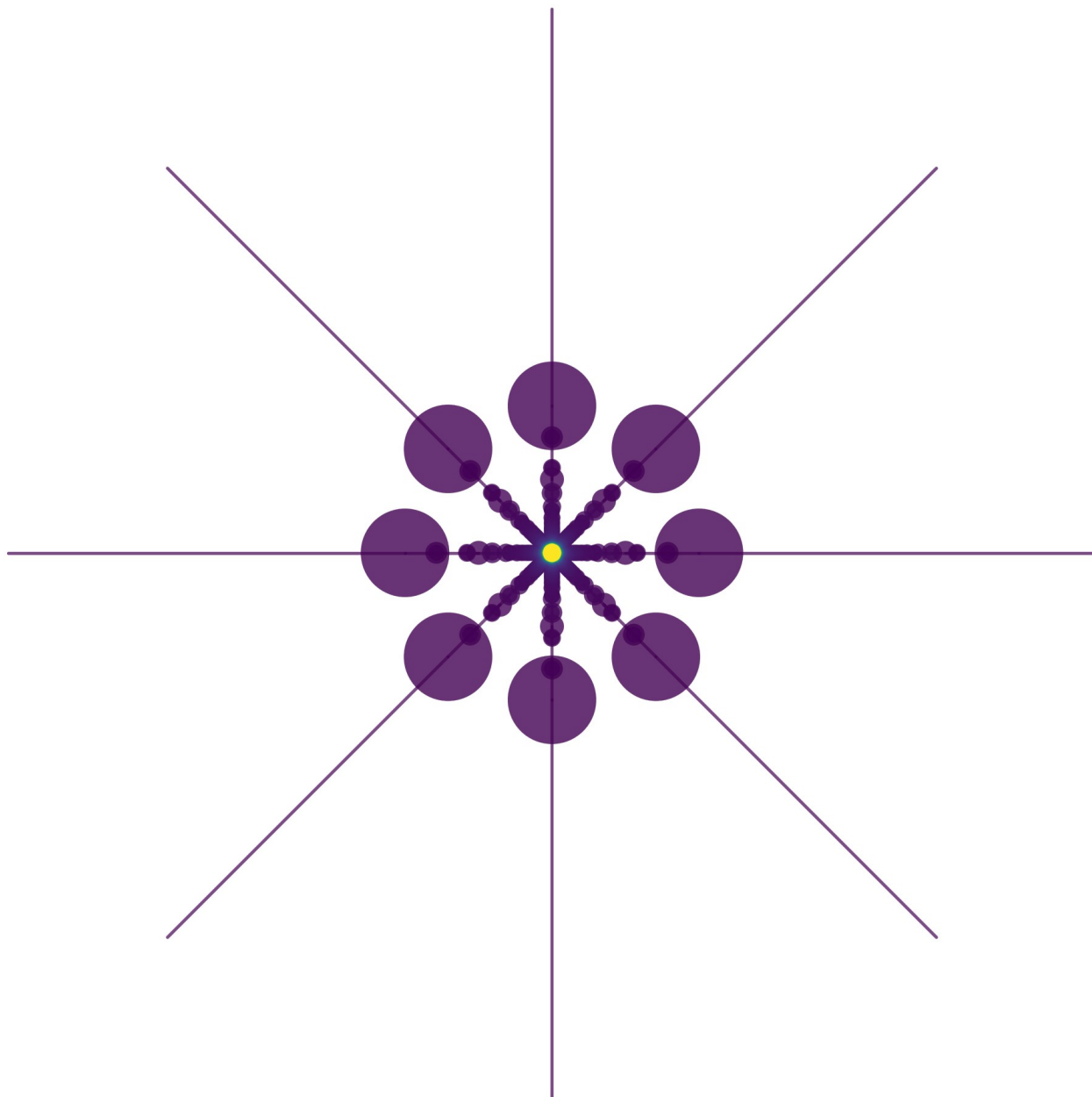
Figure 5: Generative Art from Complex Keçeci Numbers
