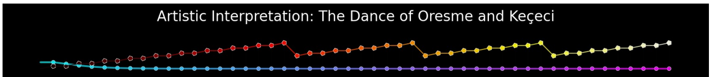
Figure 8: Artistic Interpretation: The Dance of Oresme and Keçeci Numbers
